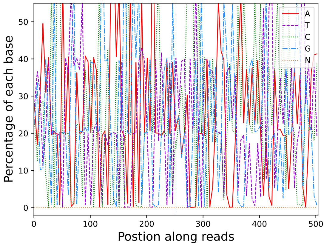
Base percentage along reads (R10117)
